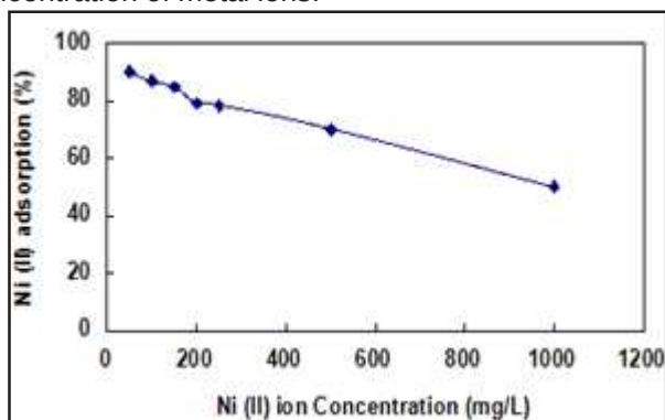
Figure -4. Effect of Ni (II) ions Concentration on adsorption Isotherm Data Analysis - The relation between the amount
