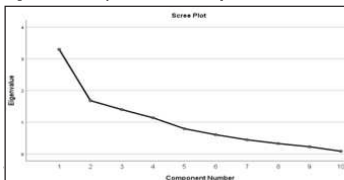
Figure 1: Scree plot of factor analysis for MLC
