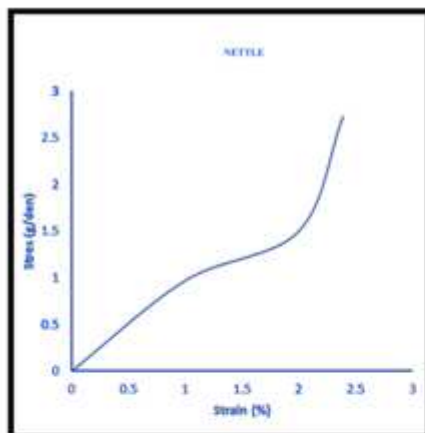
Fig.1: Representative stress-strain curve of Nettle
