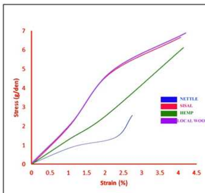
Fig. 5 : Stress-strain curve of all fibres
