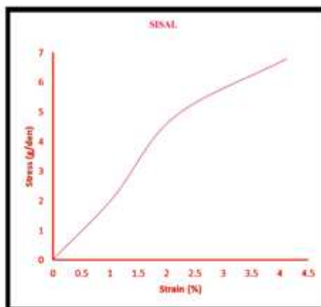
Fig.2: Representative stress-strain curve of Sisal fibre
