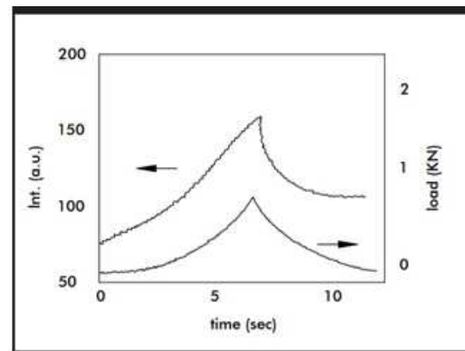
Figure 1: ML intensity dependence on rising and decreasing compressive load values on \text{SrAl}_2\text{O}_4 : Eu/Epoxy composite (based on Xu et al. ref [4])
