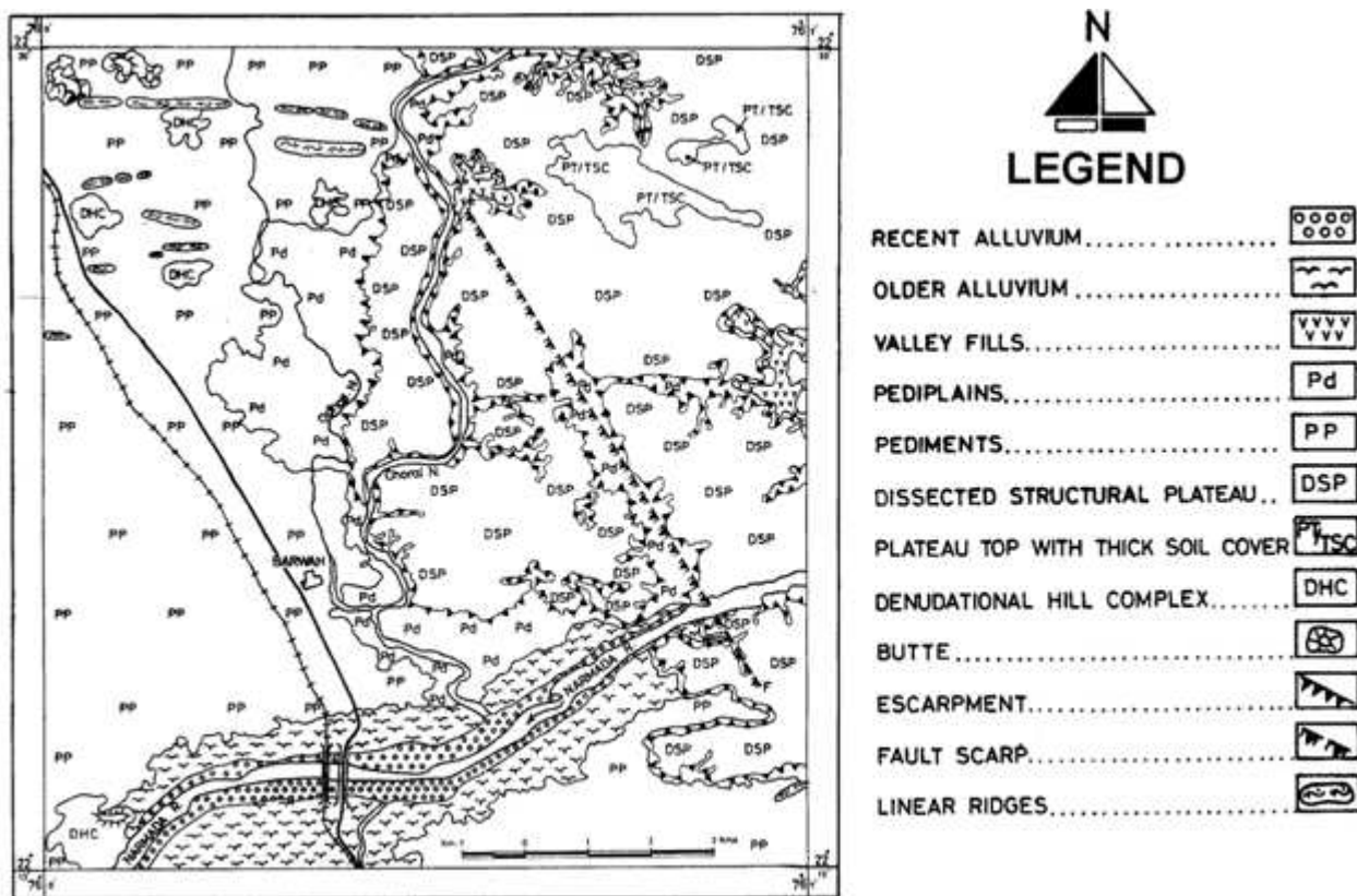
FIG. 1 GEOMORPHOLOGICAL MAP OF THE AREA
