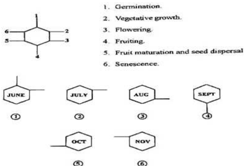
Fig. 1 : Phenograms of Indigofera linifolia showing different phenophases
